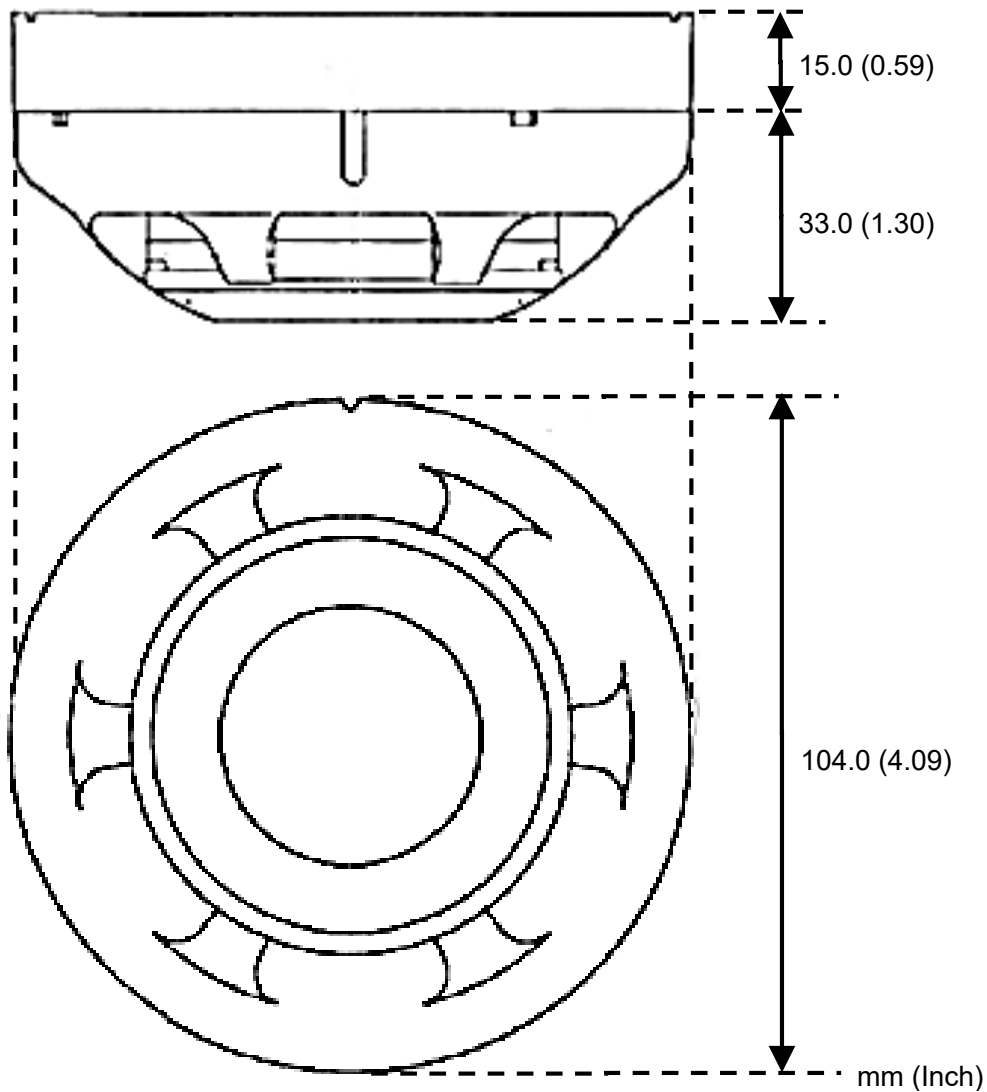
Figure1: Dimension of EVA-PY3
