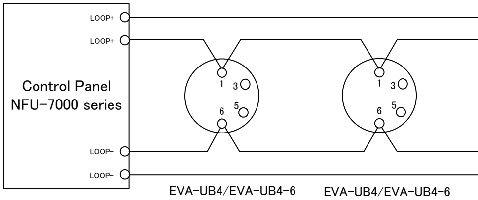
Figure 9: Wiring diagram for EVA-UB4 and EVA-UB4-6
