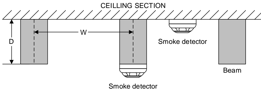
Figure 5: Smoke detector spacing — beam construction (side view)
